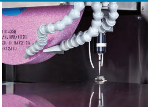
On-Board Measuring Touch Probe
