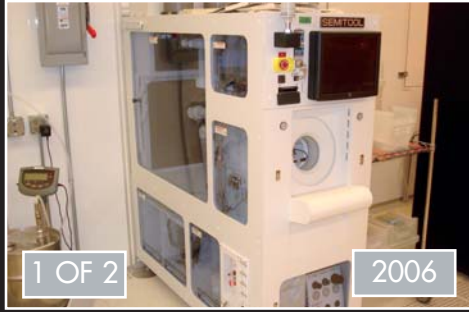
SEMITOOL MODEL SAT III & SCEPTER WET ACID TOOL ETCHERS
