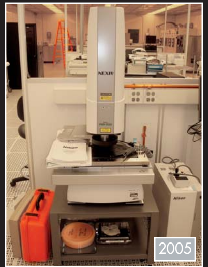
NIKON NEX1V CNC VIDEO MEASURING SYSTEM MODEL VMR-3020, VIRTUAL AUTO MEASURE
