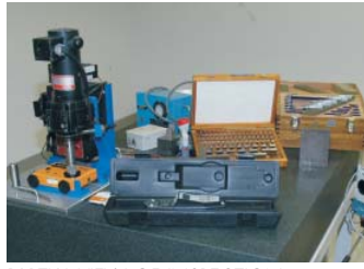
PARTIAL VIEW OF INSPECTION GAUGES- MICHIGAN
